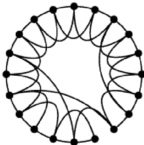
Small-world
